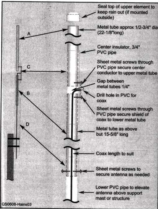
Figure 3 — Details of radome construction.
